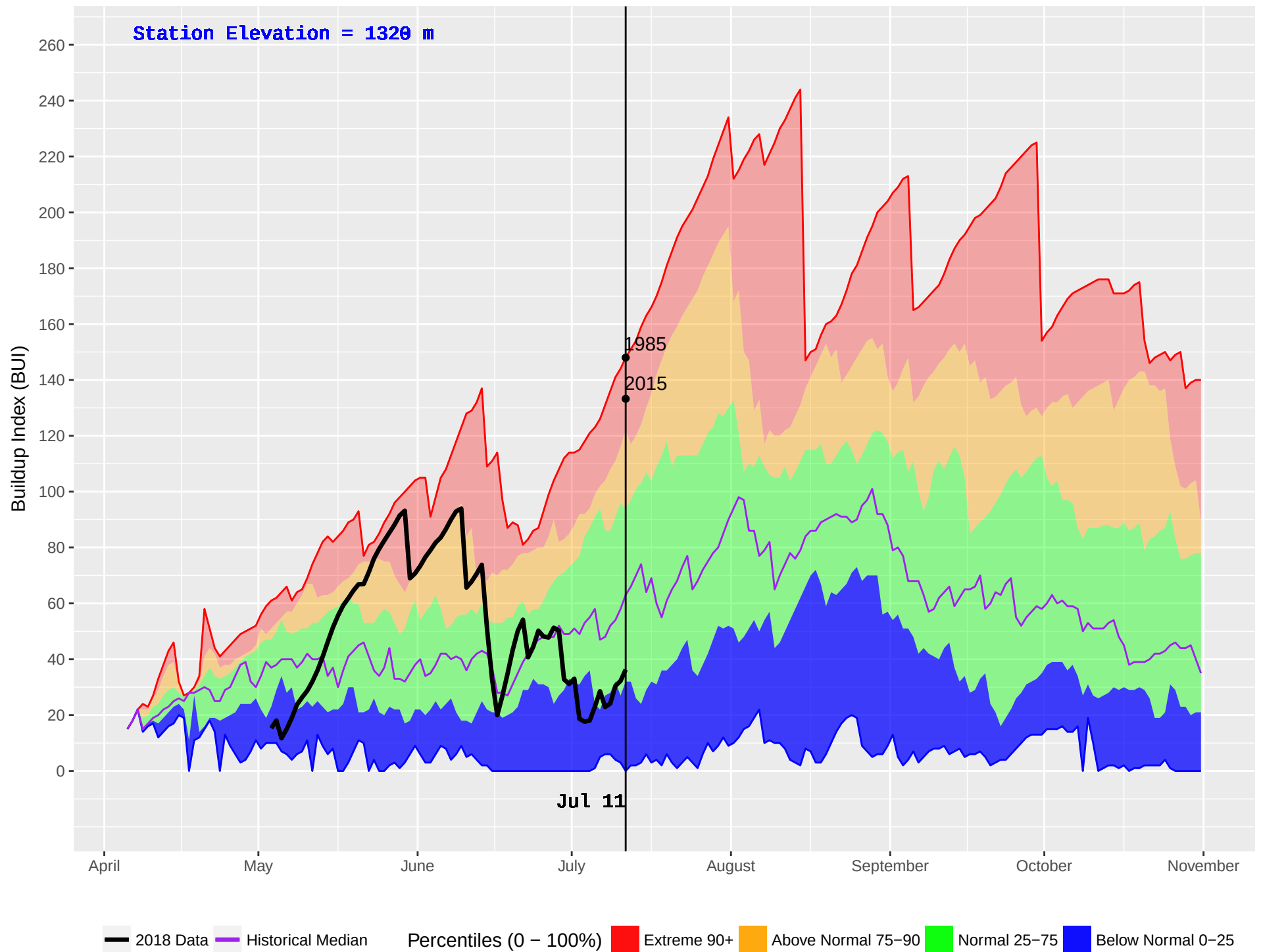
FRENCH BAR (306) : Historical (1979–2016) and Current (2018) Noon Buildup Index (BUI)
