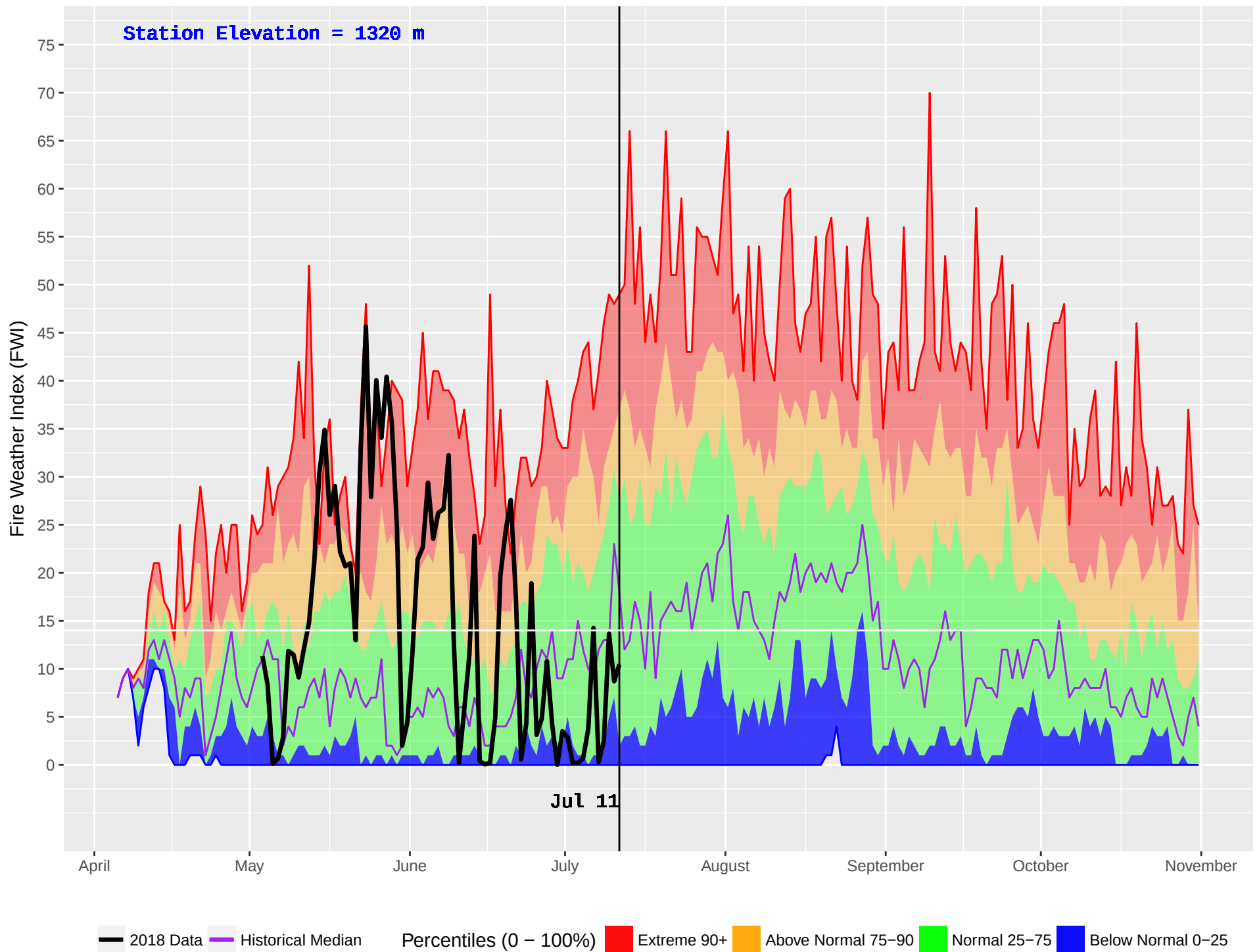
FRENCH BAR (306) : Historical (1979–2016) and Current (2018) Noon Fire Weather Index (FWI)
